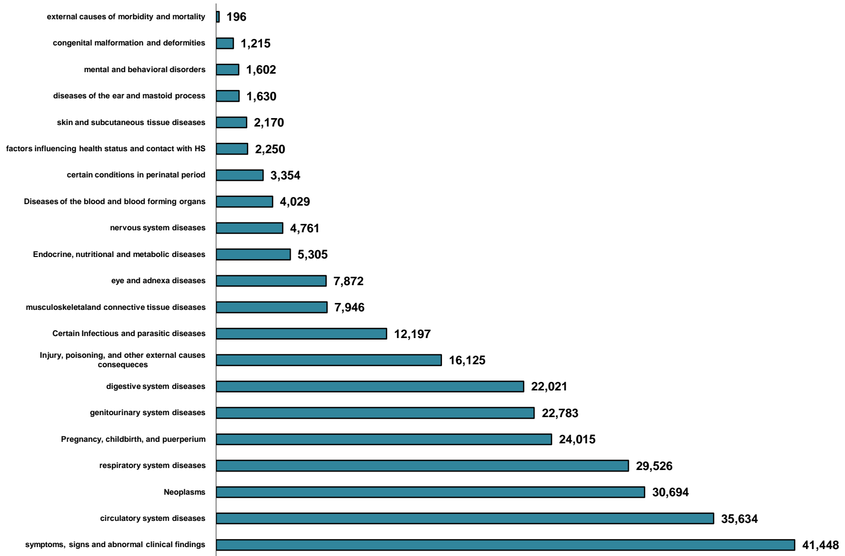
Graph C.5: MOPH subsidized admissions by ICD10 categories of diagnosis, 2013 (N=276,773)
